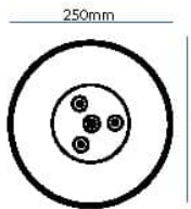
1240-1245
